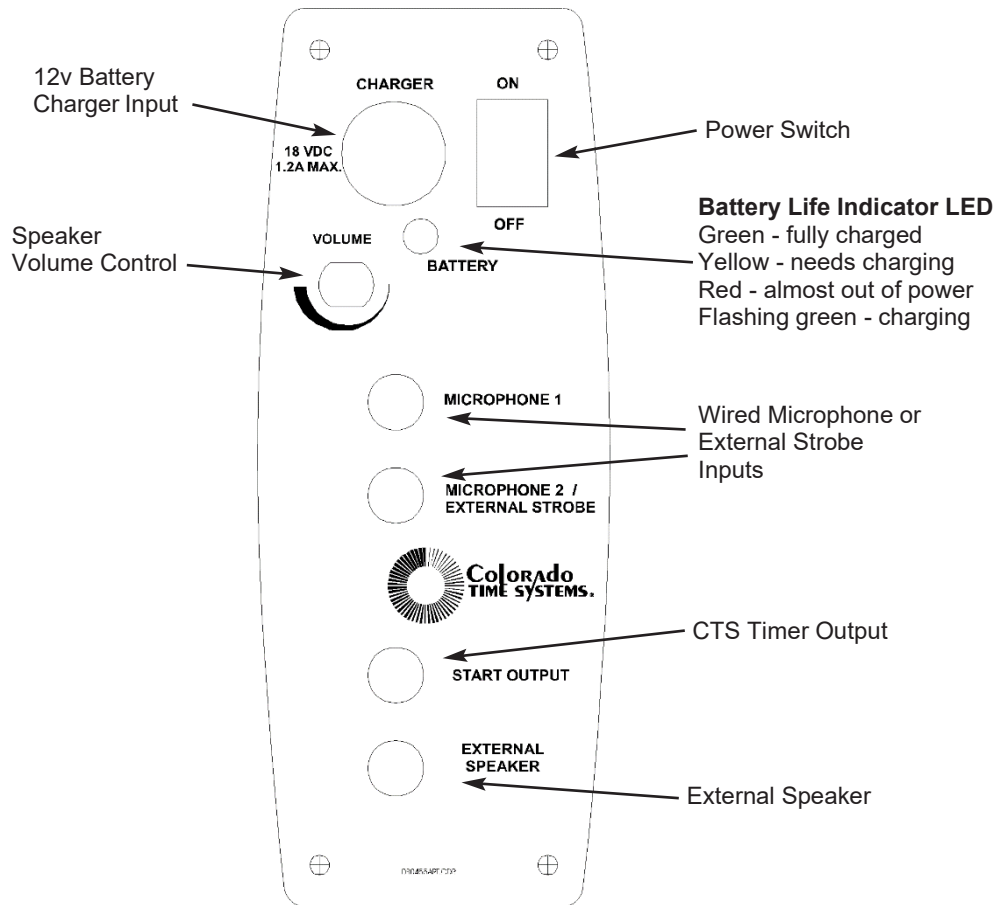
Figure B: Infinity Connection Panel
